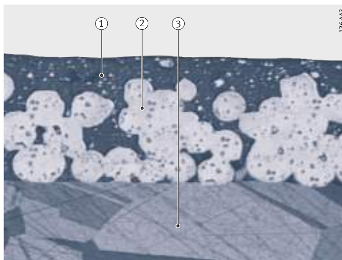
Figure 2 Permaglide® P11
