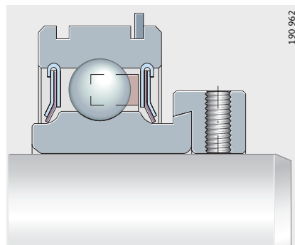
Figure 9 Radial insert ball bearings with cylindrical outer ring and two slots in outer ring
