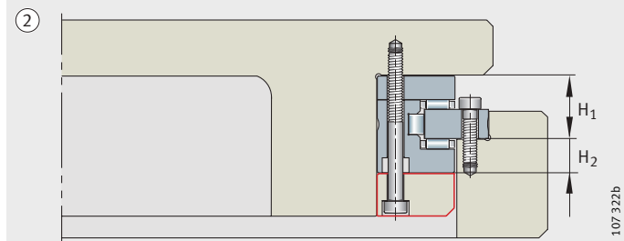
Figure 16 ① L-section ring without support ring, ② L-section ring with support ring/ for YRT, RTC
