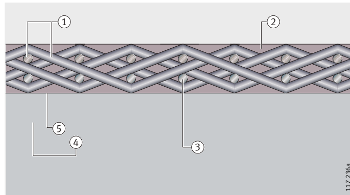
Figure 1 ELGOGLIDE ® – cross-section
