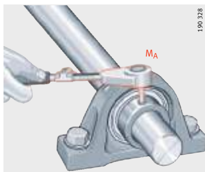
Figure 11 Tightening the grub screw in the eccentric locking collar or inner ring
