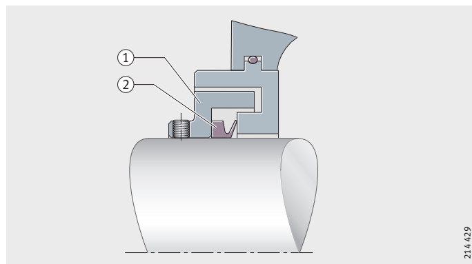
Figure 3 Example of combined seals
