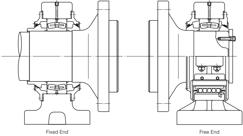
Structure of Converter Trunnion Necks
