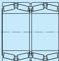
With Window Type Cages Figure 1
